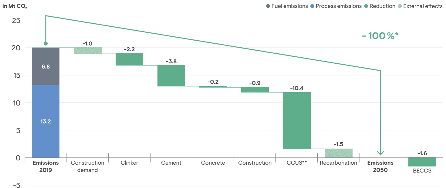
Fig. 3: Scenario climate neutrality – CO 2 reduction by 2050
